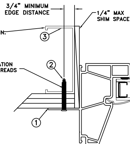
FRAME JAMB SECTION (TYP) HORIZONTAL SECTION
