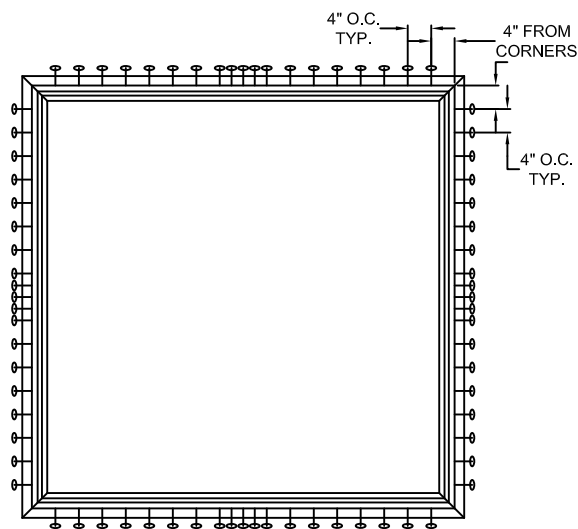
TYPICAL ELEVATION WITH FASTENER SPACING
