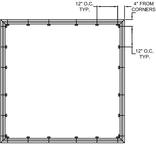
TYPICAL ELEVATION WITH FASTENER SPACING
